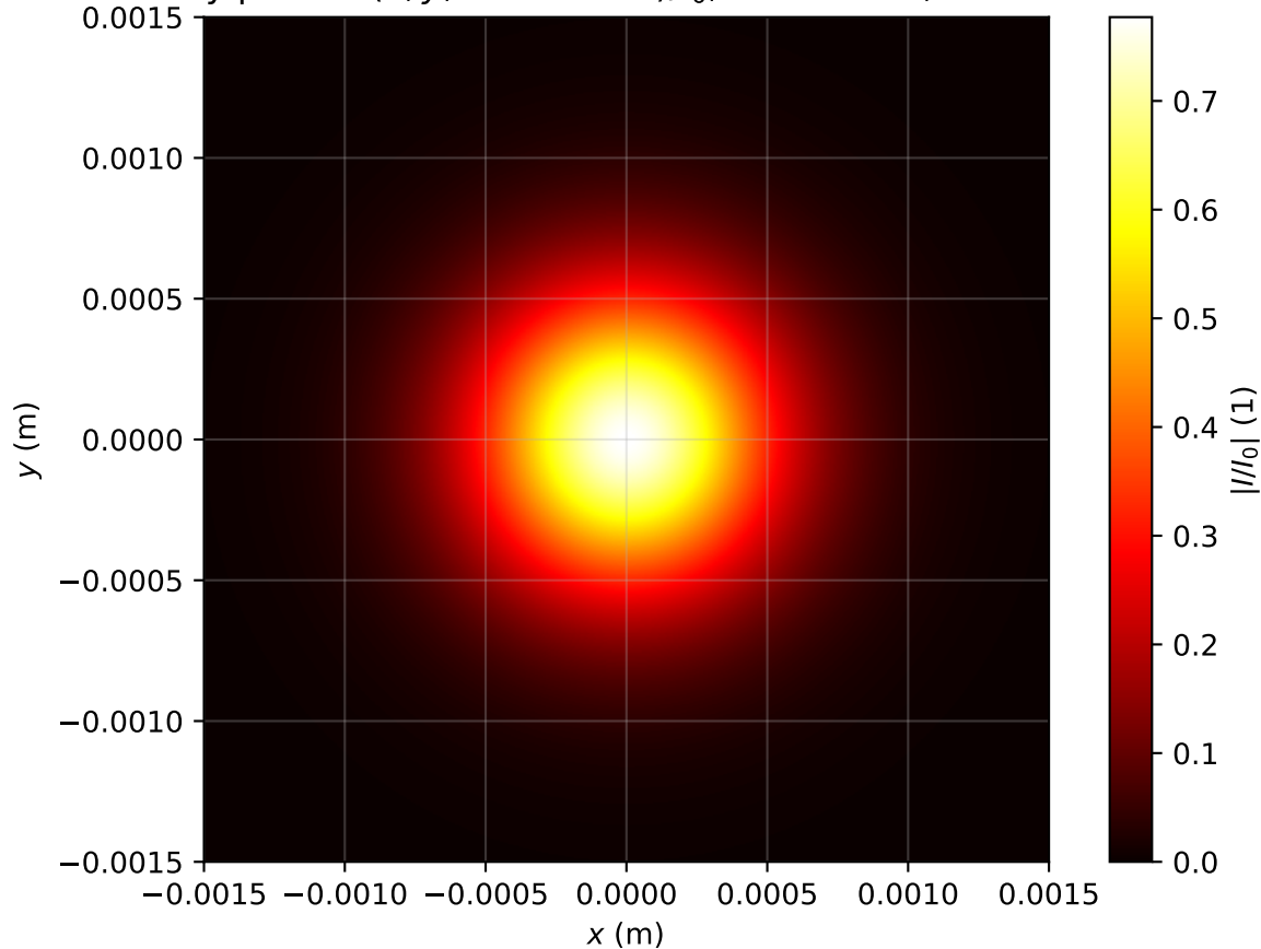
Intensity profile I(x, y, z = 1.831m)/I_0 , Pin=0.4Pcr, artificial time
